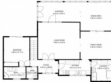
TOTAL 139 m 2 Below Ground: 90 m 2 , FLOOR 2: 141 m 2
